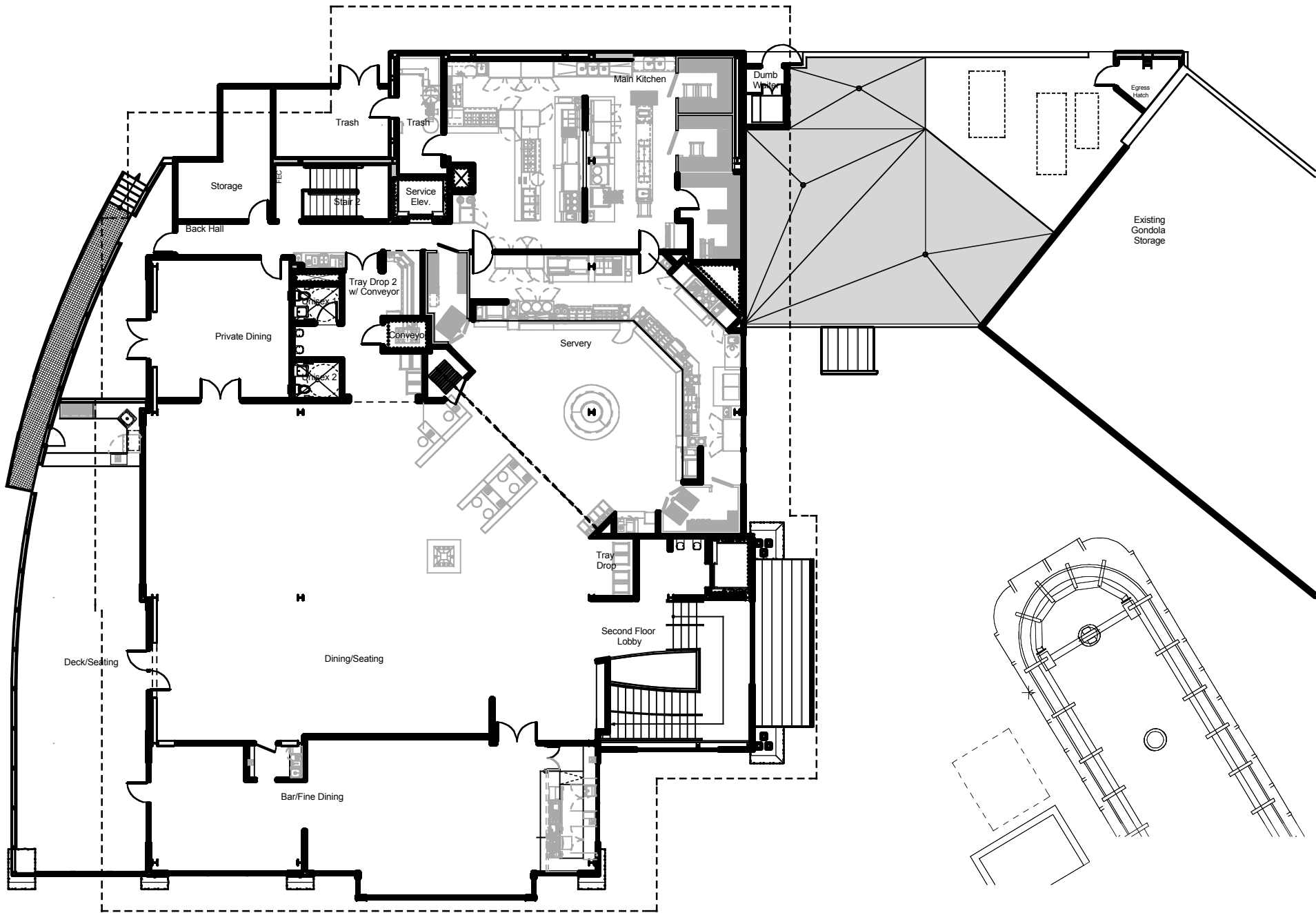
1 Level Two Floor Plan Scale: 1" = 20'
